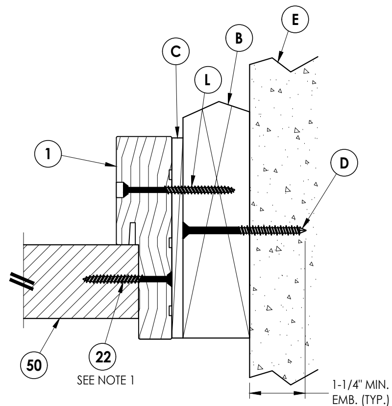
4 HORIZONTAL CROSS SECTION 3 Inswing
