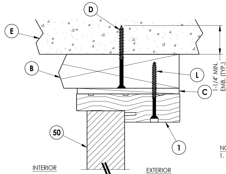
2 VERTICAL CROSS SECTION 3 Inswing
