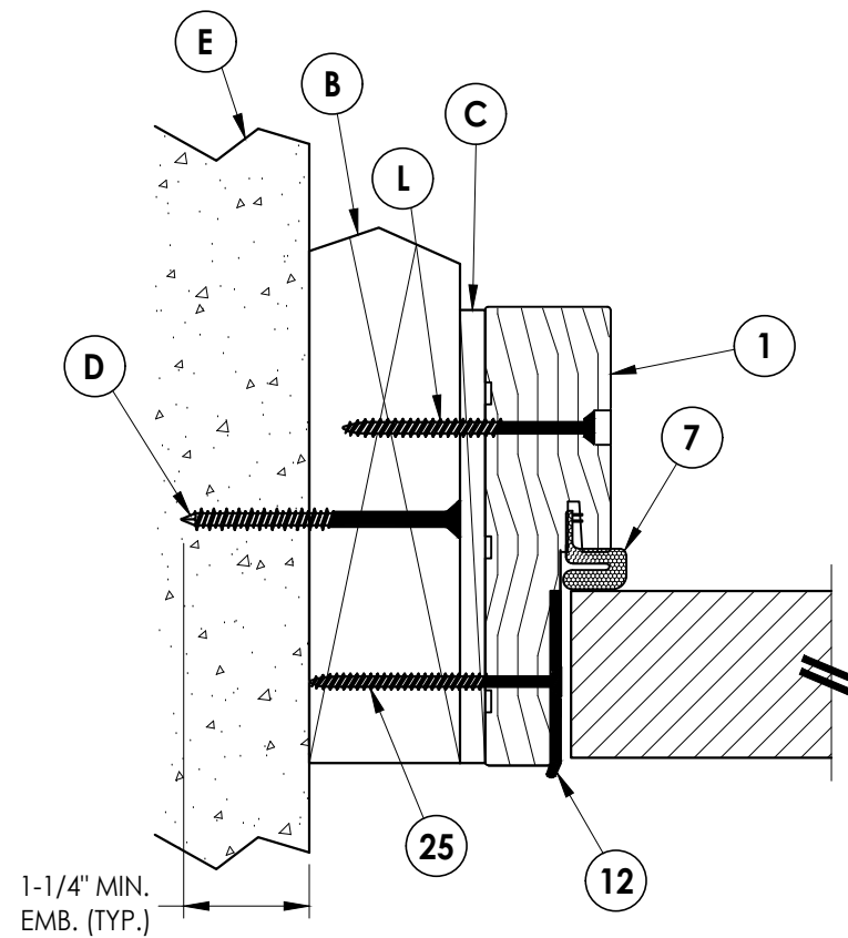
3 HORIZONTAL CROSS SECTION 3 Inswing
