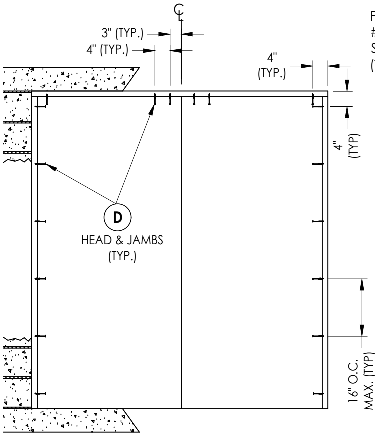
XO/OX 2X BUCK ANCHORING
