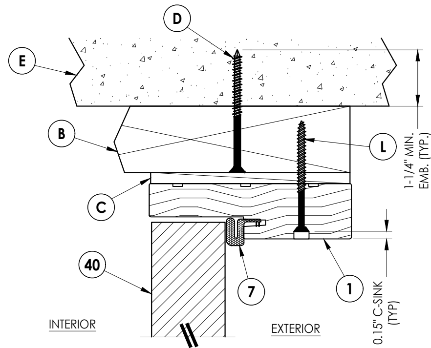
1 3 VERTICAL CROSS SECTION Inswing
